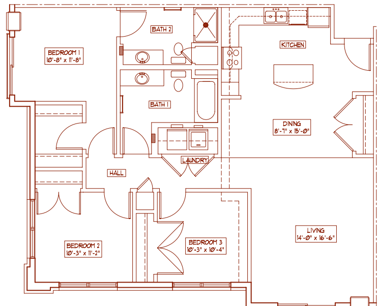
THREE BEDROOM 1335 square feet
